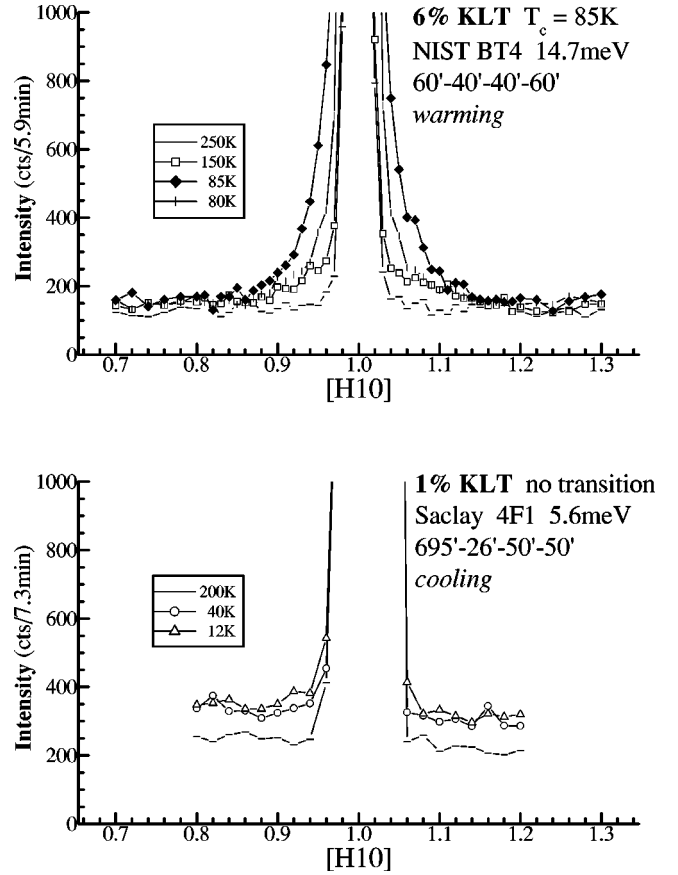
FIG. 2. Elastic scans at the (110) reciprocal point in 6 and 1% KLT single crystals. As in the 13% KLT (Fig. 1), the diffuse scattering in the 6% KLT is maximum at 85 K, below which the Bragg intensity increases. The 1% KLT crystal did not display any diffuse scattering or increase of Bragg intensity but only an increase in background.
